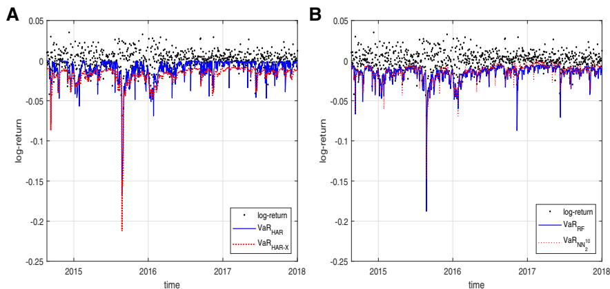
Figure 9 VaR for Apple. (A) HAR and HAR-X. (B) RF and NN_2^{10} .
