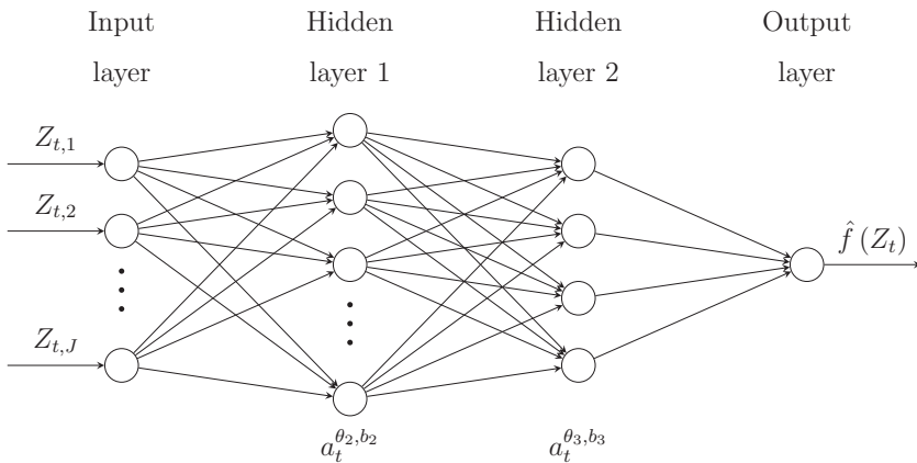
Figure 2 Feed-forward NN.
