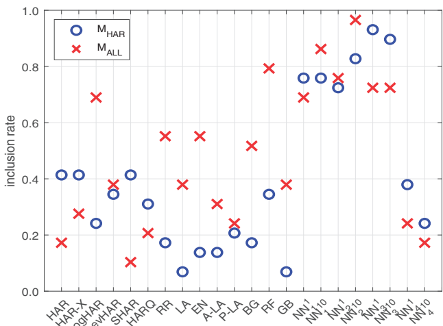
Figure 4 Inclusion rate in the MCS.
